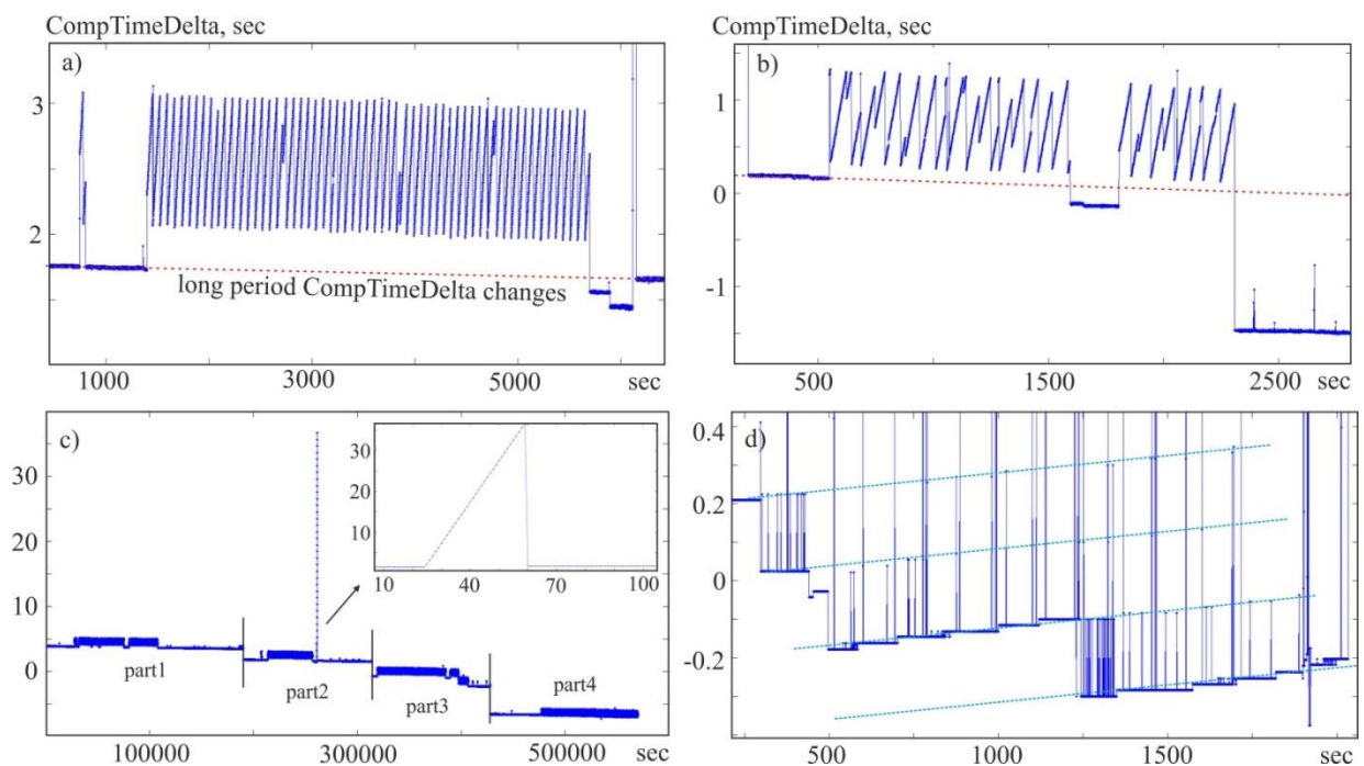
Figure 4.1 Example of difference between [GpsDay,GpsTime] and [ComputerDay,ComputerTime] in seconds (based on Geometrics MagLog files), GGA string come from Qinsy through serial port
