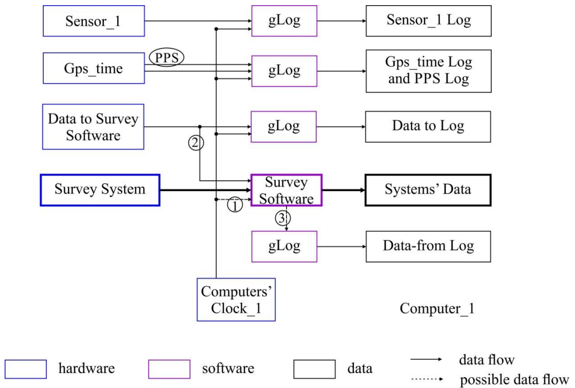
Figure 1.2 Data acquisition scheme
